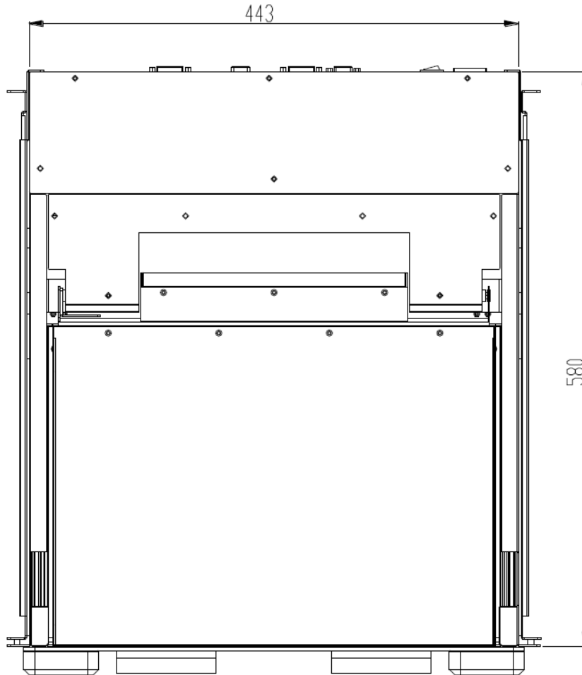
Rear of KVM-1701W-D2
